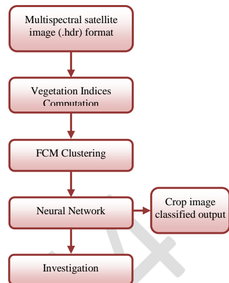
Fig.1. Flow diagram of the proposed methodology
