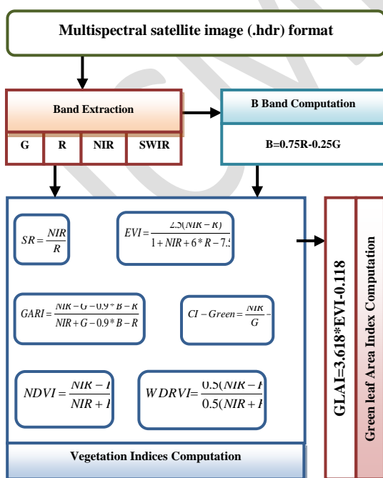
Fig.2. Computation of vegetation indices and leaf area index
