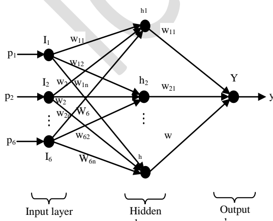
Fig.4. Pixel-based classification through Feed forward neural network
