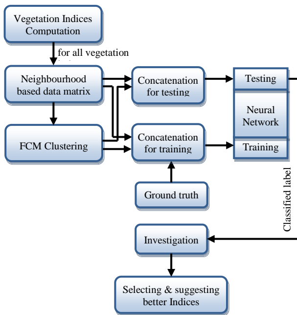
Fig.3. Steps of Crop image classification
